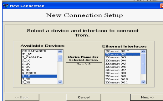
Figura 6.256 Interfaz ethernet 0/2 del switch S_1E
