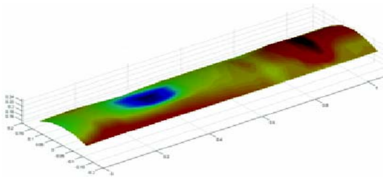
Figura 3.8 Grafica de resultado del análisis de la pared de un ducto Fuente :Thomas Beuker and Dr. Florian Rahe High-quality Smart-pig Inspection of Dents , Compliant with the US Code of Federal Regulations www.ROSEN.com
