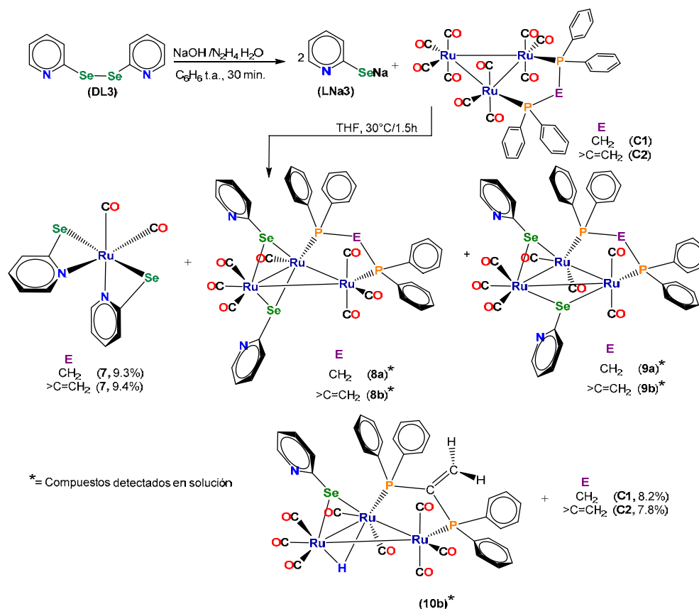
Esquema 4.1. Reactividad de los cúmulos [\text{Ru}_3(\text{CO})_{10}(\mu\text{-dppm})] ( C1 ) [\text{Ru}_3(\text{CO})_{10}(\mu\text{-dppee})] ( C2 ) con el piridil-2-selenolato de sodio LNa3 .
